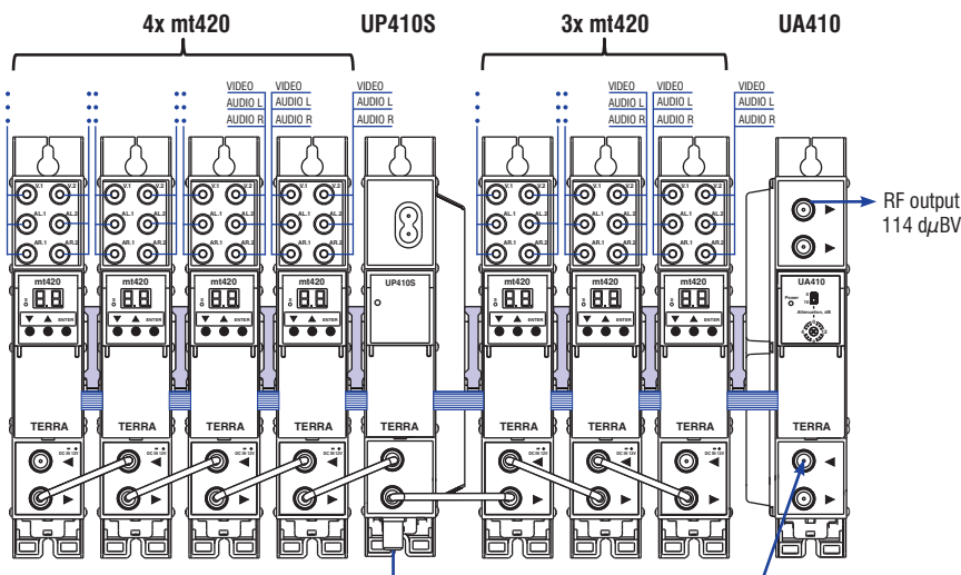
Application diagram of transmitting of 14 analog TV channels.
